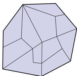
polygonal disk
