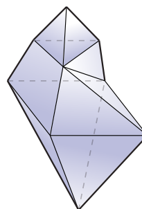
polyhedron
