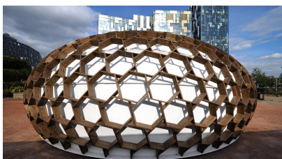
Figure 35: The hexagonal pattern exhibited by the KREOD pavilions is derived from the dual of a triangle mesh with the ball-packing property, leading to nice nodes and an even distribution of hexagons (image: KREOD).
