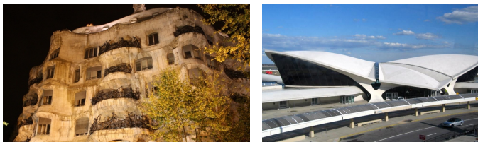
Figure 17: An early 20th century freeform geometry shaped in masonry is the 1910 Casa Milà in Barcelona by Antonio Gaudí (Photo at left by Kyle Taylor). Later, freeform shapes were realized at a grander scale in concrete, such as the TWA flight centre at JFK airport by Sarinen in 1962 (right).
