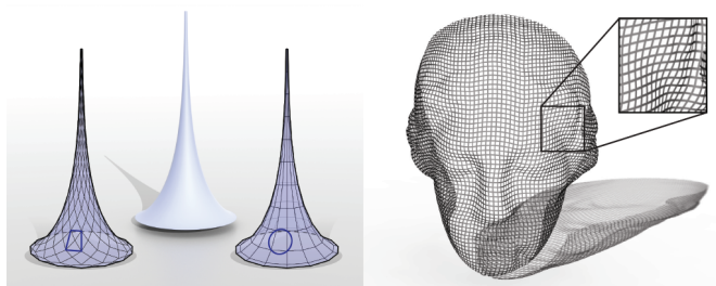
Figure 6. Left: two discrete parameterizations of a pseudosphere (constant Gauß curvature K = -1 ), one with a Chebyshev net along asymptotic directions (left) and another along principal curvature lines (right). Right: a discrete Chebyshev net on a surface of varying curvature, resembling the weft and warp directions of a woven material.
