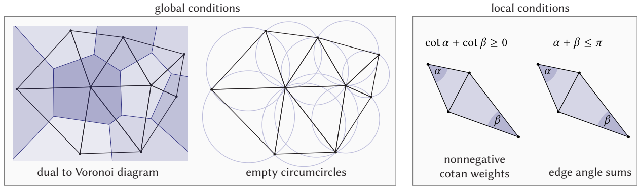
Fig. 22. There are many equivalent characterizations of the Delaunay triangulation. Here we illustrate a few examples.
