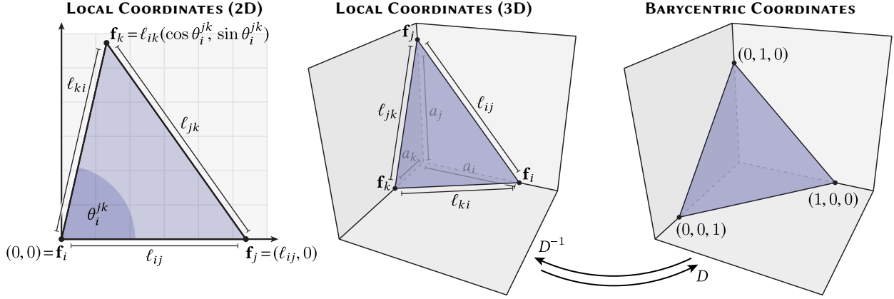
Fig. 13. Given the three edge lengths of a triangle \ell_{ij}, \ell_{jk}, \ell_{ki} , one can always find a corresponding set of vertex positions \mathbf{f}_i, \mathbf{f}_j, \mathbf{f}_k in either 2D or 3D. If the vertices of the 3D embedding are placed along the principal axes, then they are related to the barycentric coordinates by a simple diagonal scaling D .
