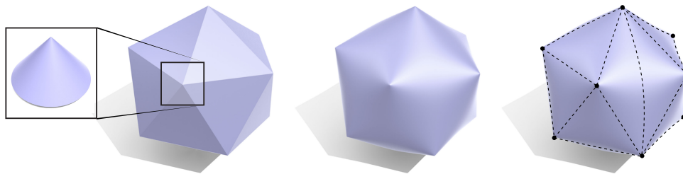
Fig. 12. Left: intrinsically, a small neighborhood around any vertex of a polyhedral surface is indistinguishable from a round circular cone. For instance, a vertex made from triangular pieces of paper can be easily smoothed out into a circular cone without stretching or ripping. Center: a good mental “cartoon” of an intrinsic triangulation is hence a surface where the edges are completely smooth, and only the vertices are visible. Right: from this perspective, no one triangulation is special—there are many intrinsic triangulations that describe the exact same geometry.
