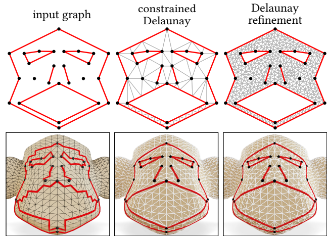
Fig. 25. Top . Planar constrained Delaunay triangulations are used to produce high-quality triangulations which conform to a collection of specified lines. Bottom . Constrained intrinsic triangulations play a similar role on surfaces, preserving a set of intrinsic edges in the triangulation.
