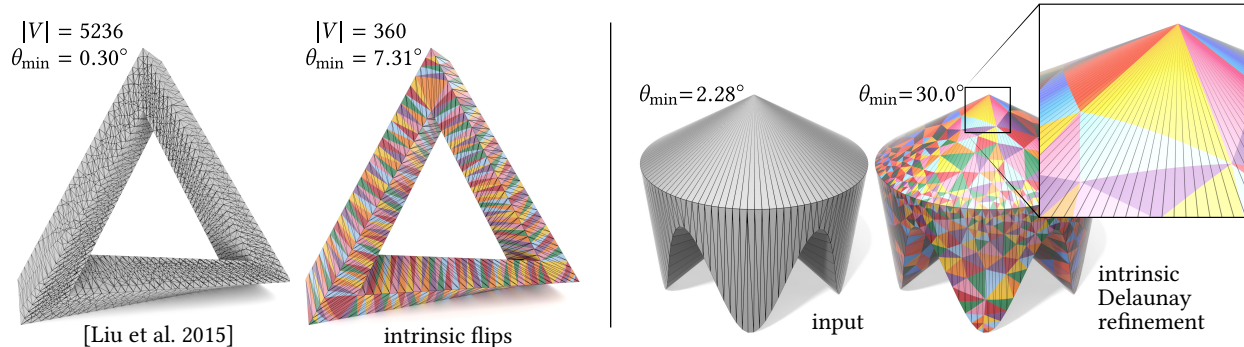
Fig. 28. Left : Extrinsic schemes may need to insert many vertices and create skinny triangles to produce a Delaunay triangulation while preserving the shape, while the intrinsic approach preserves the vertex set and improves triangles quality. Right : Small corner angles in an extrinsic triangulation must remain if extrinsic shape is to be preserved, but instead preserving only the intrinsic shape allows these angles to be improved.
