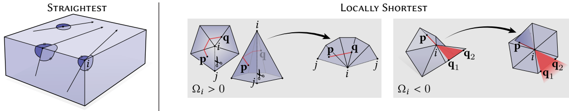
Fig. 16. There are two distinct ways to define geodesics on polyhedra: as “straightest” curves, with equal angle on both sides ( left ), or as “locally shortest” curves that cannot be pulled tighter ( right ). A curve through a positively-curved vertex ( \Omega_i > 0 ) can always be made shorter, whereas there are many ways to continue a path through a negatively-curved vertex ( \Omega_i < 0 ) while remaining locally shortest—for example, a path from p through i and then to either q_1 or q_2 is locally shortest. For intrinsic triangulations, we need only consider locally shortest geodesics. ( Leftmost figure adapted from [Polthier and Schmieß 2006] )
