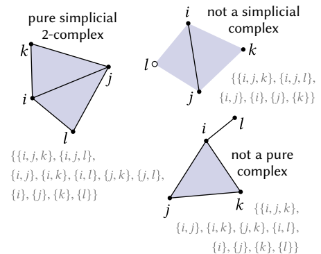
Fig. 5. In a simplicial complex, an edge must have two distinct endpoints, and a triangle must have three distinct vertices.
