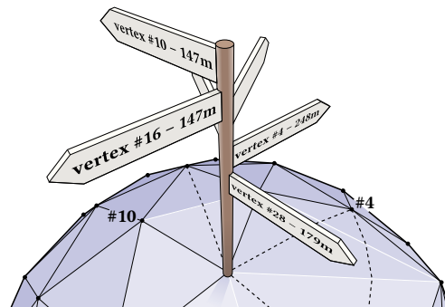
Fig. 20. Signposts encode edges of an intrinsic by storing the length and direction of each edge in the tangent space each vertex.
