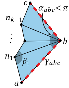
Fig. 34. Notation for FLIPOUT.
